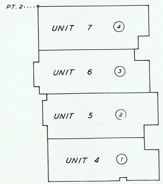
FIRST FLOOR BUILDING 2
